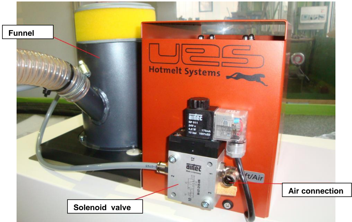
Solenoid valve and air connection mounted externally outside of the pump dome
